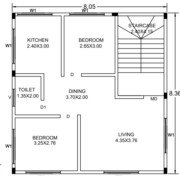
TYP: FIRST & SECOND FLOOR PLAN
